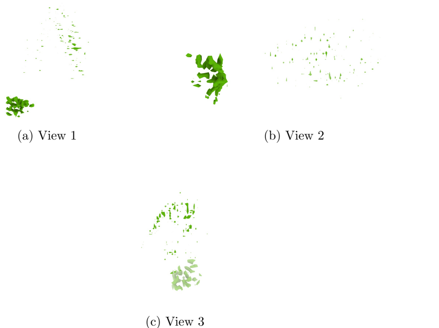
Figure 4: Isosurface at threshold=0.200000. Views generated by ChimeraX at a the following X, Y, Z angles: View 1 (0, -90, -90), View 2 (-90, 0, -90), View 3 (0, 0, 0).
