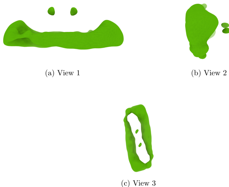
Figure 4: Isosurface at threshold=0.100000. Views generated by ChimeraX at a the following X, Y, Z angles: View 1 (0, -90, -90), View 2 (-90, 0, -90), View 3 (0, 0, 0).
