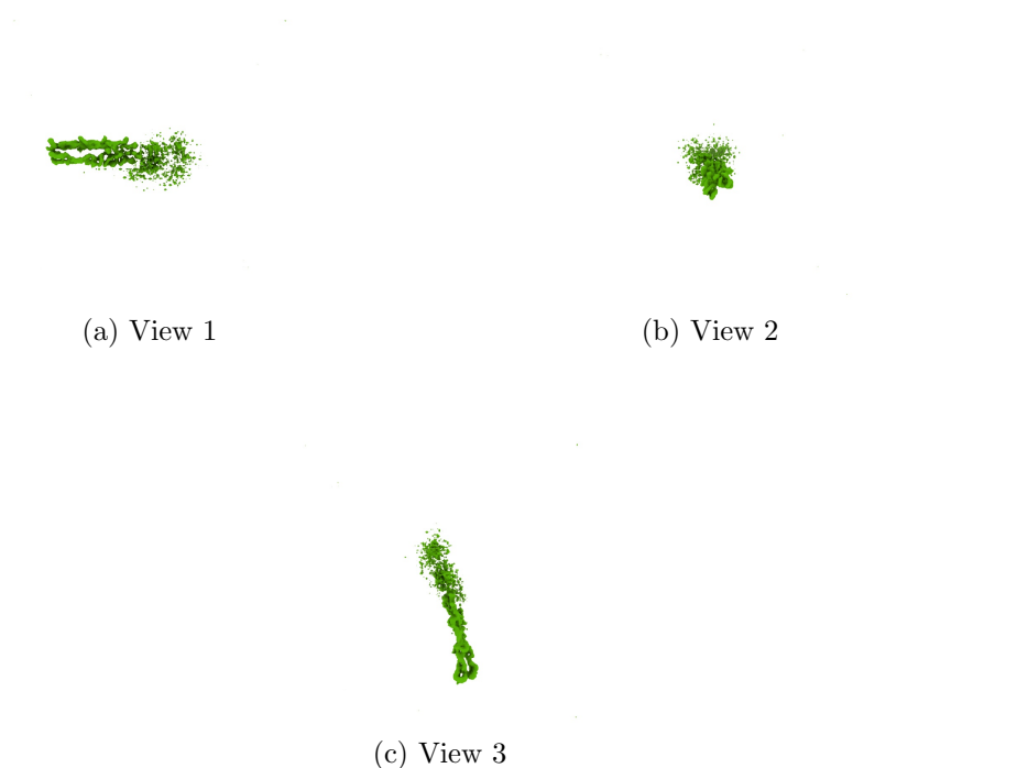
Figure 4: Isosurface at threshold=0.110000. Views generated by ChimeraX at a the following X, Y, Z angles: View 1 (0, -90, -90), View 2 (-90, 0, -90), View 3 (0, 0, 0).
