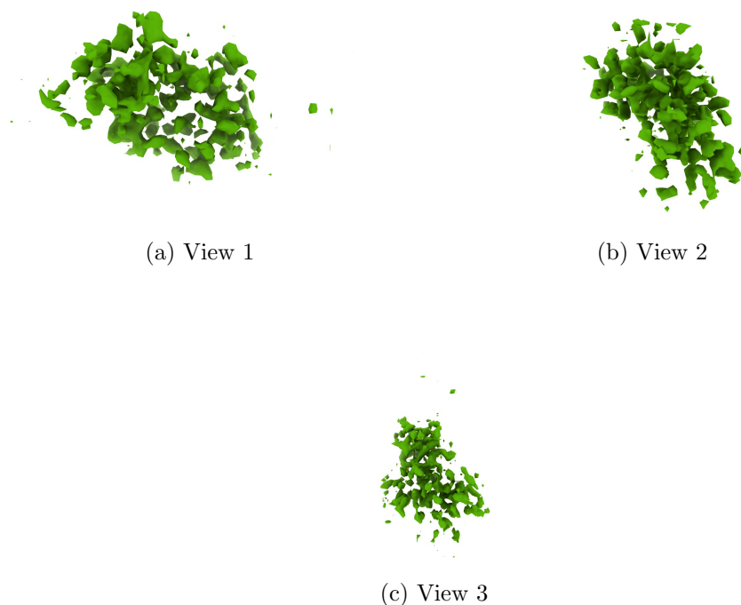
Figure 4: Isosurface at threshold=0.075000. Views generated by ChimeraX at a the following X, Y, Z angles: View 1 (0, -90, -90), View 2 (-90, 0, -90), View 3 (0, 0, 0).
