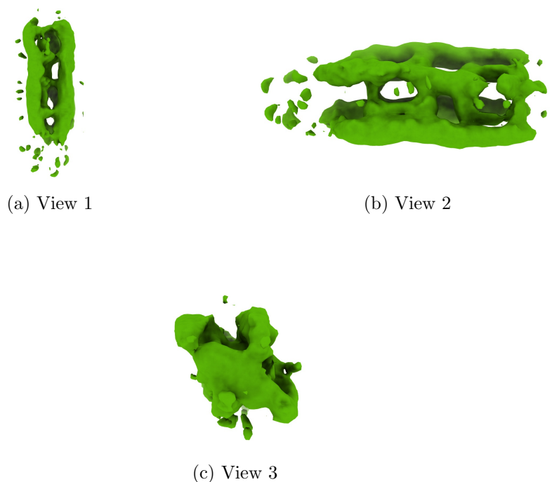
Figure 4: Isosurface at threshold=0.073800. Views generated by ChimeraX at a the following X, Y, Z angles: View 1 (0, -90, -90), View 2 (-90, 0, -90), View 3 (0, 0, 0).
