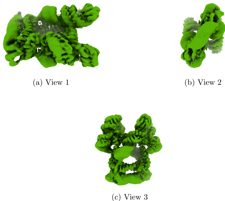
Figure 4: Isosurface at threshold=0.001100. Views generated by ChimeraX at a the following X, Y, Z angles: View 1 (0, -90, -90), View 2 (-90, 0, -90), View 3 (0, 0, 0).
