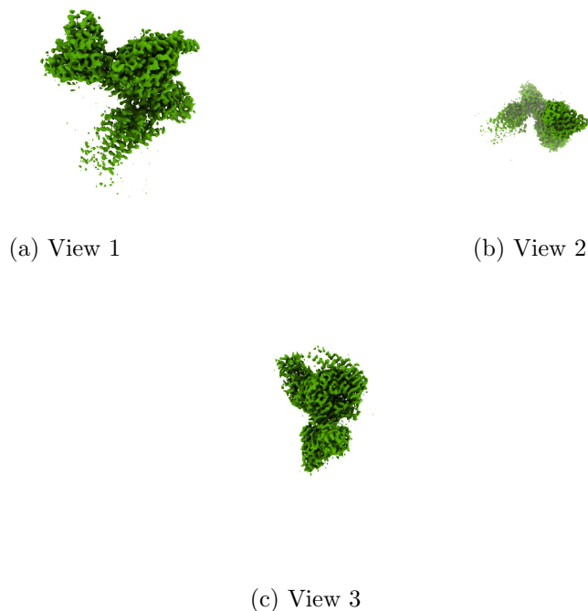
Figure 4: Isosurface at threshold=0.375000. Views generated by ChimeraX at a the following X, Y, Z angles: View 1 (0, -90, -90), View 2 (-90, 0, -90), View 3 (0, 0, 0).
