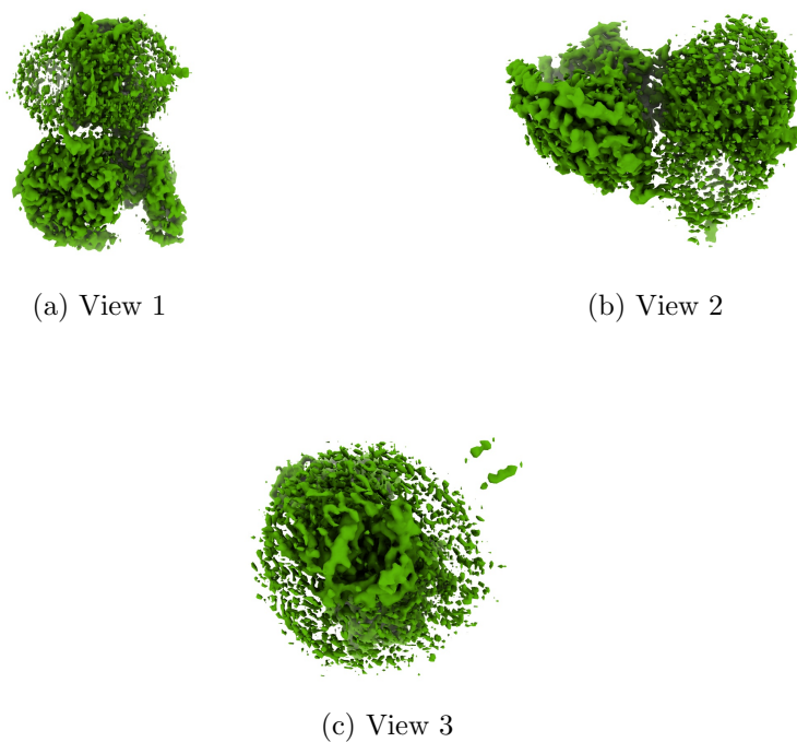
Figure 4: Isosurface at threshold=0.182000. Views generated by ChimeraX at a the following X, Y, Z angles: View 1 (0, -90, -90), View 2 (-90, 0, -90), View 3 (0, 0, 0).
