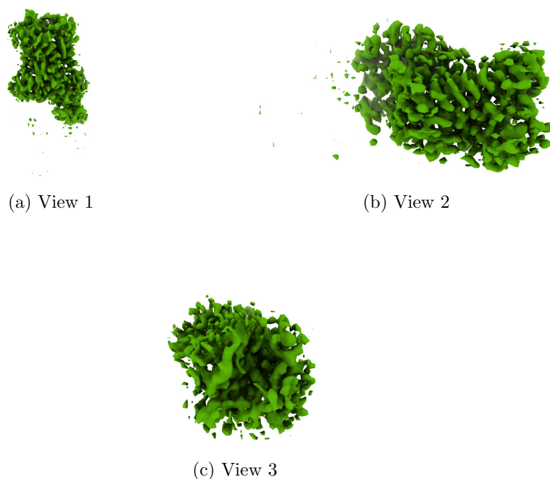
Figure 4: Isosurface at threshold=0.299000. Views generated by ChimeraX at a the following X, Y, Z angles: View 1 (0, -90, -90), View 2 (-90, 0, -90), View 3 (0, 0, 0).
