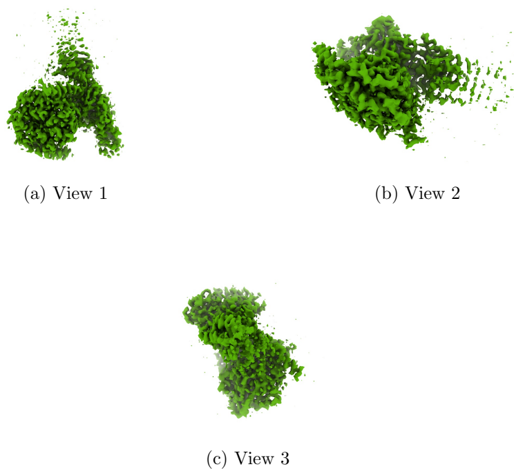
Figure 4: Isosurface at threshold=0.299000. Views generated by ChimeraX at a the following X, Y, Z angles: View 1 (0, -90, -90), View 2 (-90, 0, -90), View 3 (0, 0, 0).
