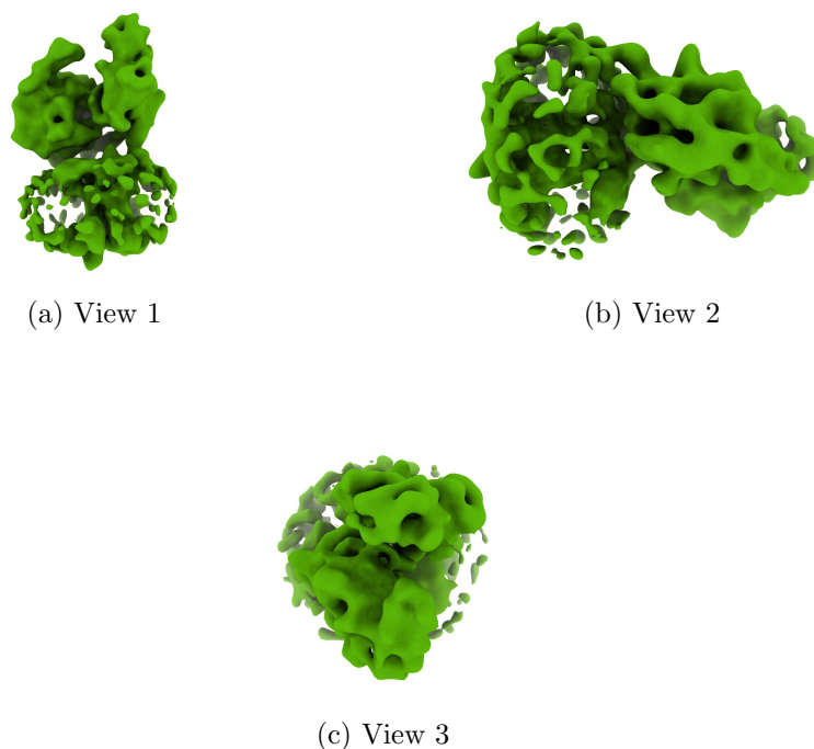
Figure 4: Isosurface at threshold=0.126000. Views generated by ChimeraX at a the following X, Y, Z angles: View 1 (0, -90, -90), View 2 (-90, 0, -90), View 3 (0, 0, 0).
