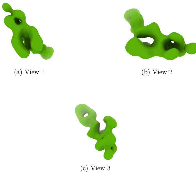
Figure 4: Isosurface at threshold=0.026300. Views generated by ChimeraX at a the following X, Y, Z angles: View 1 (0, -90, -90), View 2 (-90, 0, -90), View 3 (0, 0, 0).
