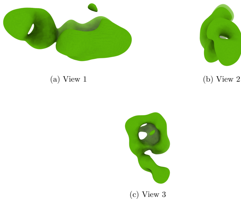
Figure 4: Isosurface at threshold=0.034100. Views generated by ChimeraX at a the following X, Y, Z angles: View 1 (0, -90, -90), View 2 (-90, 0, -90), View 3 (0, 0, 0).
