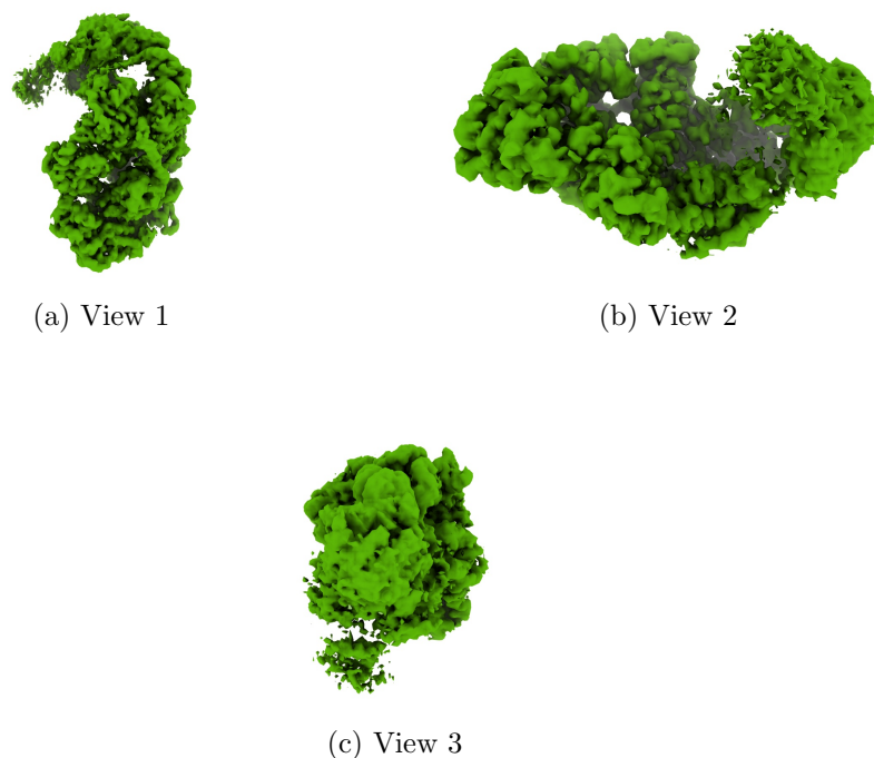
Figure 4: Isosurface at threshold=0.053000. Views generated by ChimeraX at a the following X, Y, Z angles: View 1 (0, -90, -90), View 2 (-90, 0, -90), View 3 (0, 0, 0).
