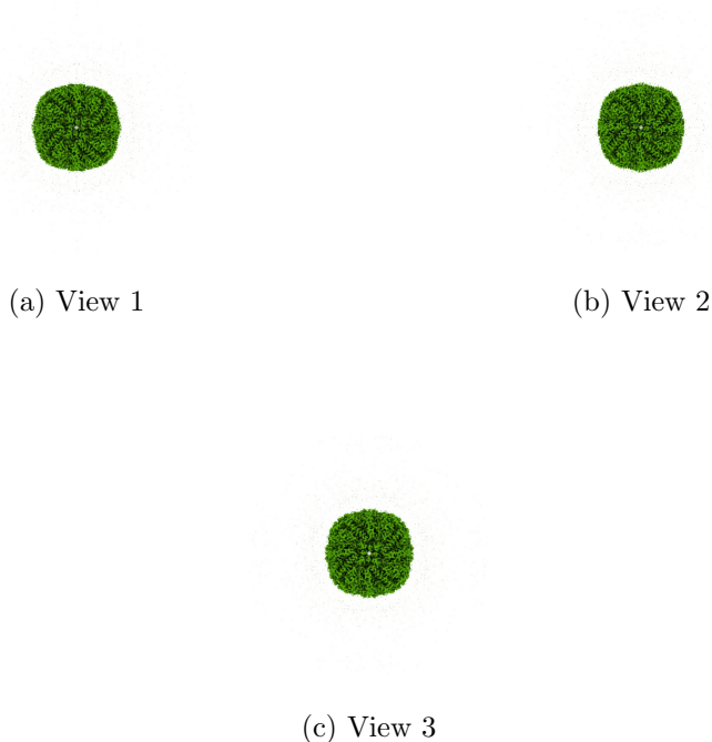
Figure 4: Isosurface at threshold=0.300000. Views generated by ChimeraX at a the following X, Y, Z angles: View 1 (0, -90, -90), View 2 (-90, 0, -90), View 3 (0, 0, 0).
