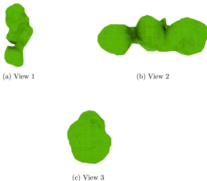
Figure 4: Isosurface at threshold=0.388000. Views generated by ChimeraX at a the following X, Y, Z angles: View 1 (0, -90, -90), View 2 (-90, 0, -90), View 3 (0, 0, 0).
