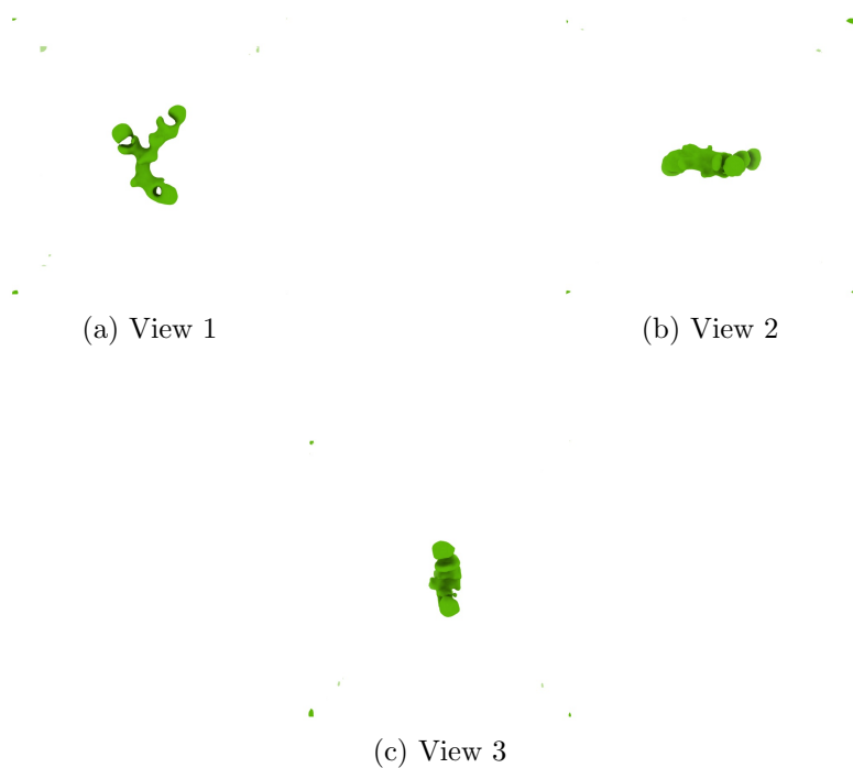
Figure 4: Isosurface at threshold=3.050000. Views generated by ChimeraX at a the following X, Y, Z angles: View 1 (0, -90, -90), View 2 (-90, 0, -90), View 3 (0, 0, 0).
