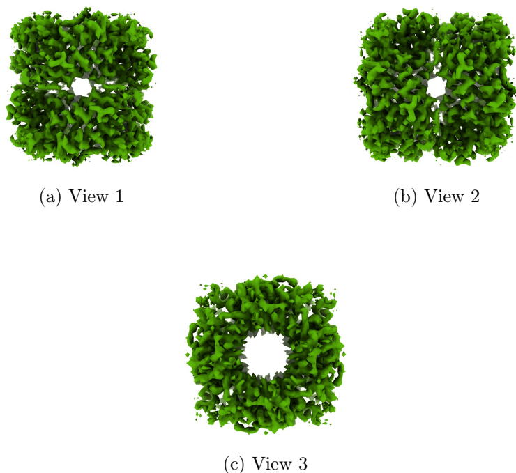
Figure 4: Isosurface at threshold=0.611000. Views generated by ChimeraX at a the following X, Y, Z angles: View 1 (0, -90, -90), View 2 (-90, 0, -90), View 3 (0, 0, 0).
