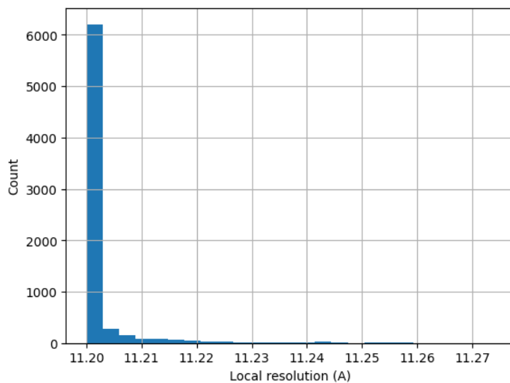
Figure 20: Histogram of the local resolution according to Resmap.
