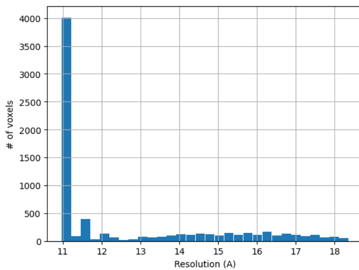
Figure 22: Histogram of the local resolution according to MonoRes.
