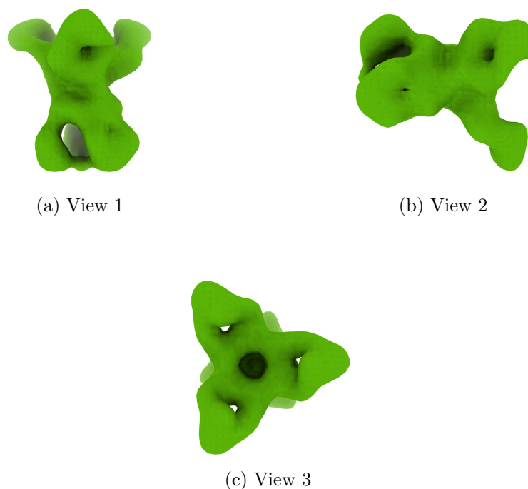
Figure 4: Isosurface at threshold=1.010000. Views generated by ChimeraX at a the following X, Y, Z angles: View 1 (0, -90, -90), View 2 (-90, 0, -90), View 3 (0, 0, 0).
