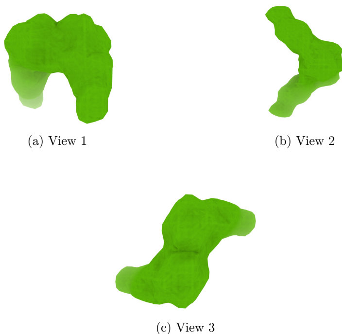
Figure 4: Isosurface at threshold=1.940000. Views generated by ChimeraX at a the following X, Y, Z angles: View 1 (0, -90, -90), View 2 (-90, 0, -90), View 3 (0, 0, 0).
