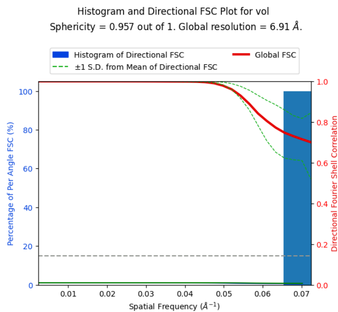
Figure 26: Global FSC and histogram of the directional FSC.
