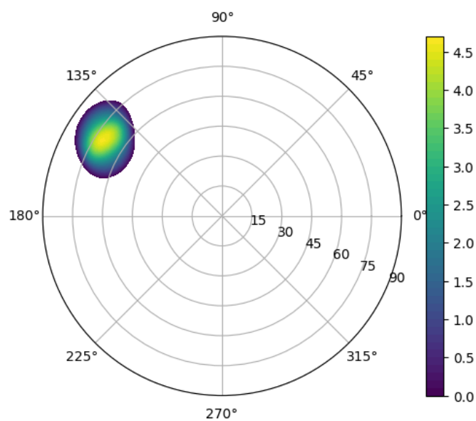
Figure 24: Directional resolution in the projection sphere.
