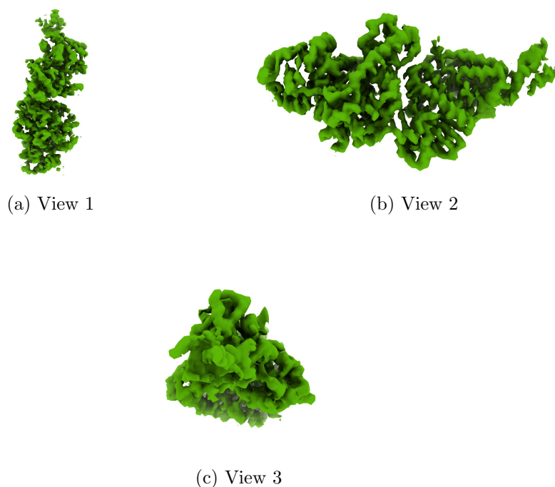
Figure 4: Isosurface at threshold=0.003500. Views generated by ChimeraX at a the following X, Y, Z angles: View 1 (0, -90, -90), View 2 (-90, 0, -90), View 3 (0, 0, 0).
