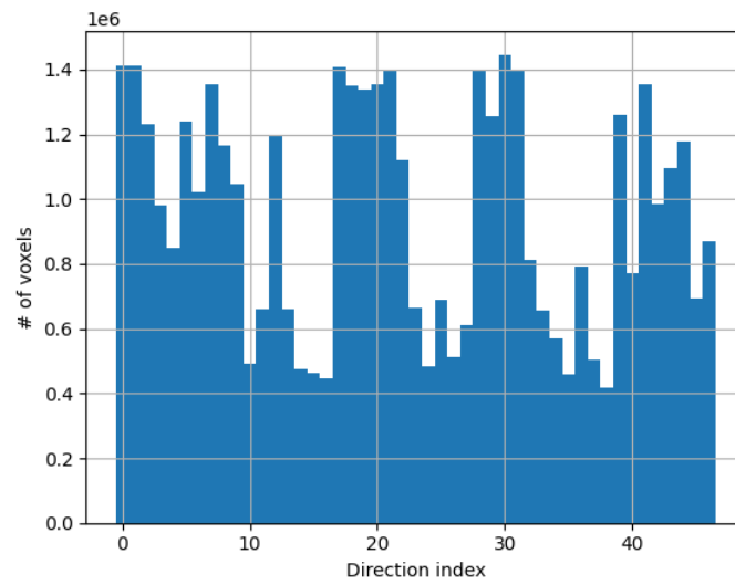
Figure 27: Histogram 1D of the best direction at each voxel.
