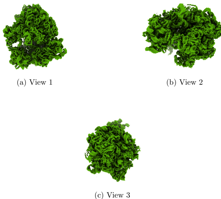
Figure 4: Isosurface at threshold=0.270000. Views generated by ChimeraX at a the following X, Y, Z angles: View 1 (0, -90, -90), View 2 (-90, 0, -90), View 3 (0, 0, 0).
