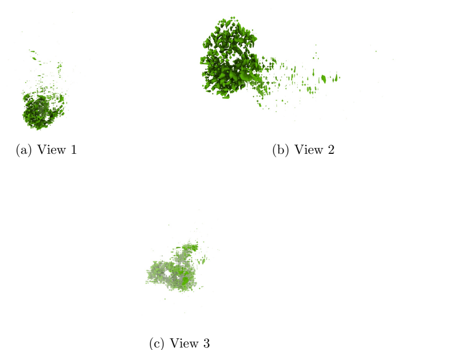
Figure 4: Isosurface at threshold=0.060000. Views generated by ChimeraX at a the following X, Y, Z angles: View 1 (0, -90, -90), View 2 (-90, 0, -90), View 3 (0, 0, 0).
