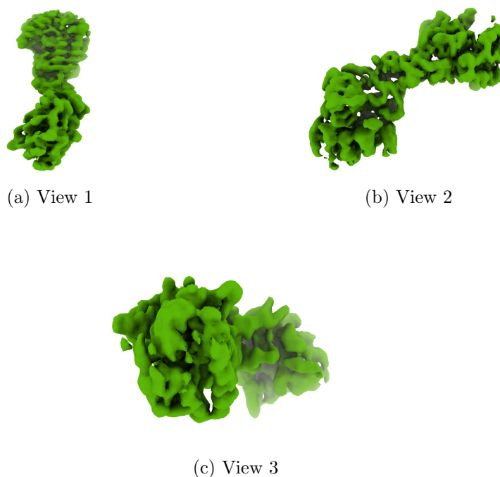
Figure 4: Isosurface at threshold=0.000500. Views generated by ChimeraX at a the following X, Y, Z angles: View 1 (0, -90, -90), View 2 (-90, 0, -90), View 3 (0, 0, 0).
