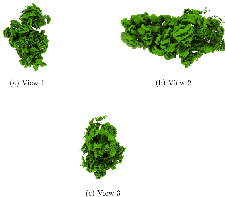
Figure 4: Isosurface at threshold=0.262000. Views generated by ChimeraX at a the following X, Y, Z angles: View 1 (0, -90, -90), View 2 (-90, 0, -90), View 3 (0, 0, 0).
