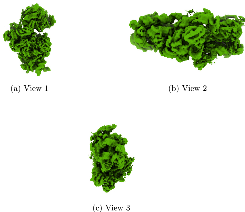
Figure 4: Isosurface at threshold=0.219000. Views generated by ChimeraX at a the following X, Y, Z angles: View 1 (0, -90, -90), View 2 (-90, 0, -90), View 3 (0, 0, 0).
