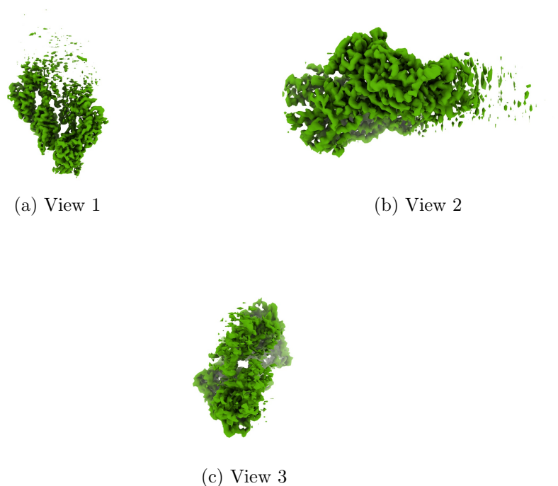
Figure 4: Isosurface at threshold=0.057500. Views generated by ChimeraX at a the following X, Y, Z angles: View 1 (0, -90, -90), View 2 (-90, 0, -90), View 3 (0, 0, 0).
