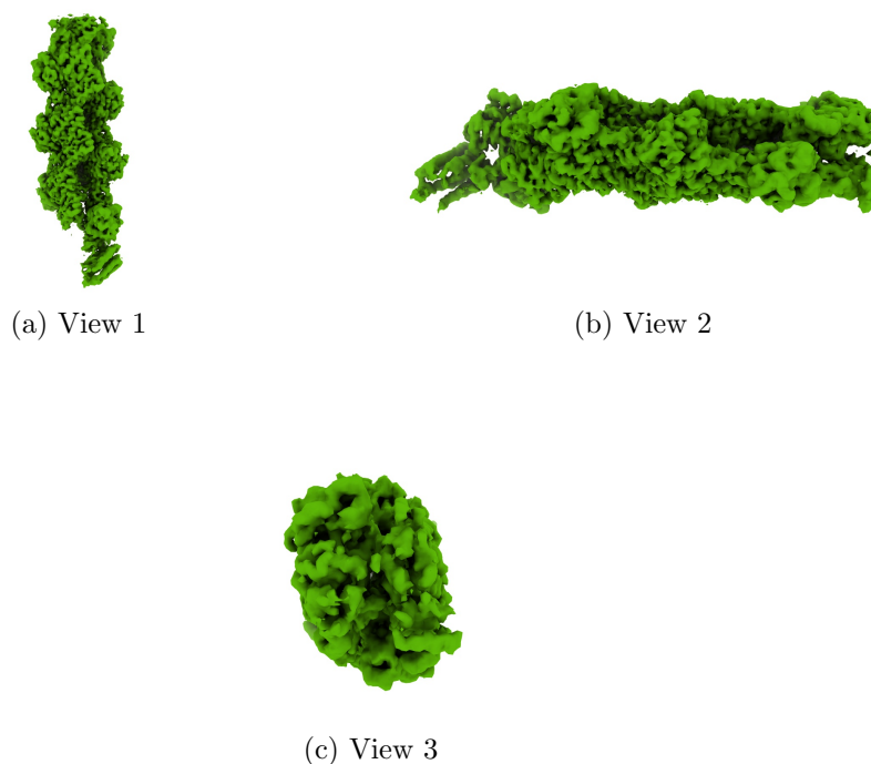
Figure 4: Isosurface at threshold=0.028100. Views generated by ChimeraX at a the following X, Y, Z angles: View 1 (0, -90, -90), View 2 (-90, 0, -90), View 3 (0, 0, 0).
