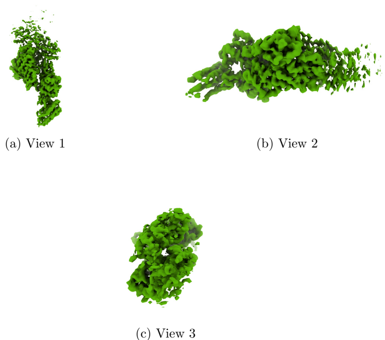
Figure 4: Isosurface at threshold=0.039300. Views generated by ChimeraX at a the following X, Y, Z angles: View 1 (0, -90, -90), View 2 (-90, 0, -90), View 3 (0, 0, 0).
