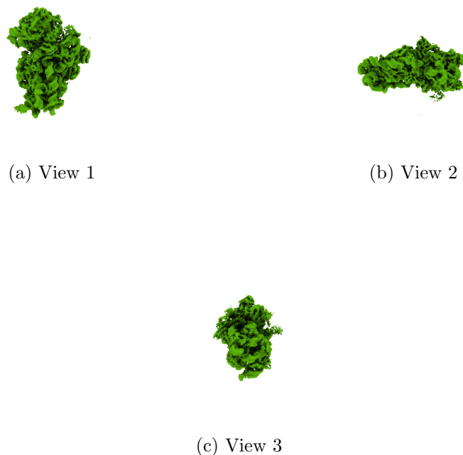
Figure 4: Isosurface at threshold=0.238000. Views generated by ChimeraX at a the following X, Y, Z angles: View 1 (0, -90, -90), View 2 (-90, 0, -90), View 3 (0, 0, 0).
