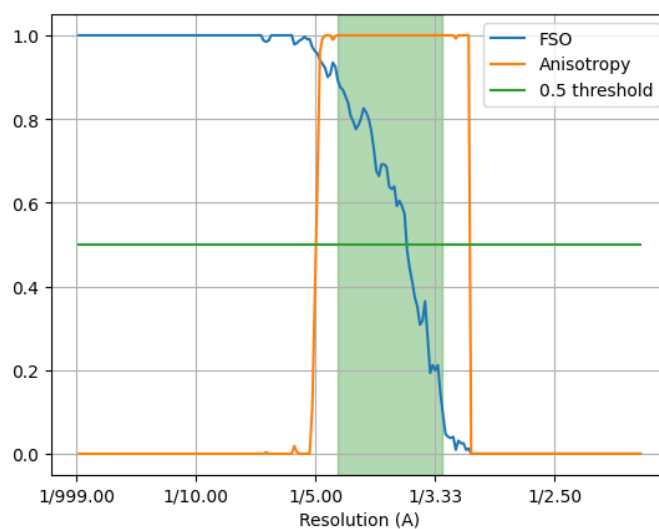
Figure 27: FSO and anisotropy.
