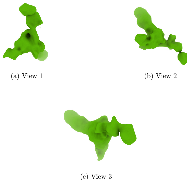
Figure 4: Isosurface at threshold=0.067600. Views generated by ChimeraX at a the following X, Y, Z angles: View 1 (0, -90, -90), View 2 (-90, 0, -90), View 3 (0, 0, 0).
