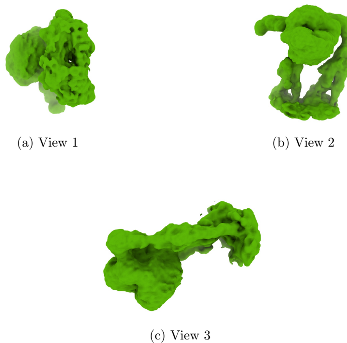
Figure 4: Isosurface at threshold=0.000486. Views generated by ChimeraX at a the following X, Y, Z angles: View 1 (0, -90, -90), View 2 (-90, 0, -90), View 3 (0, 0, 0).
