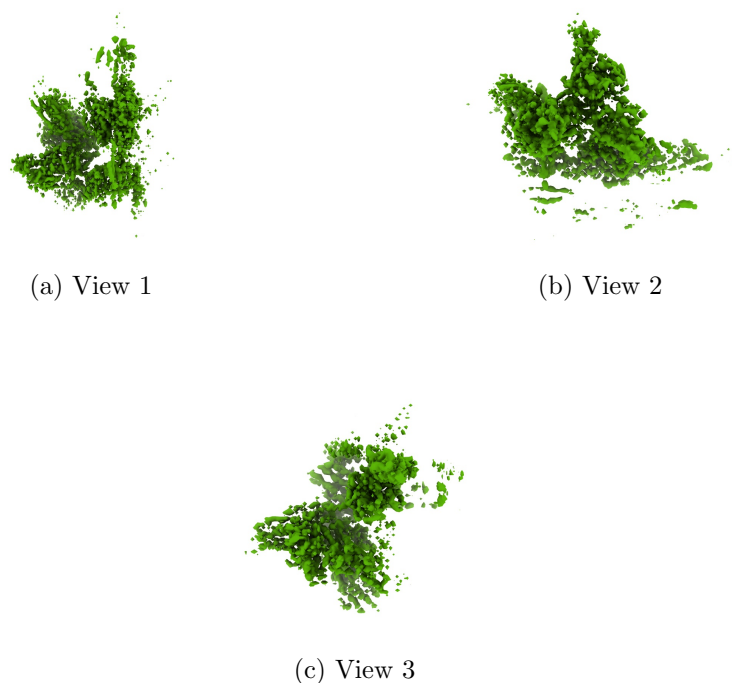
Figure 4: Isosurface at threshold=0.155000. Views generated by ChimeraX at a the following X, Y, Z angles: View 1 (0, -90, -90), View 2 (-90, 0, -90), View 3 (0, 0, 0).
