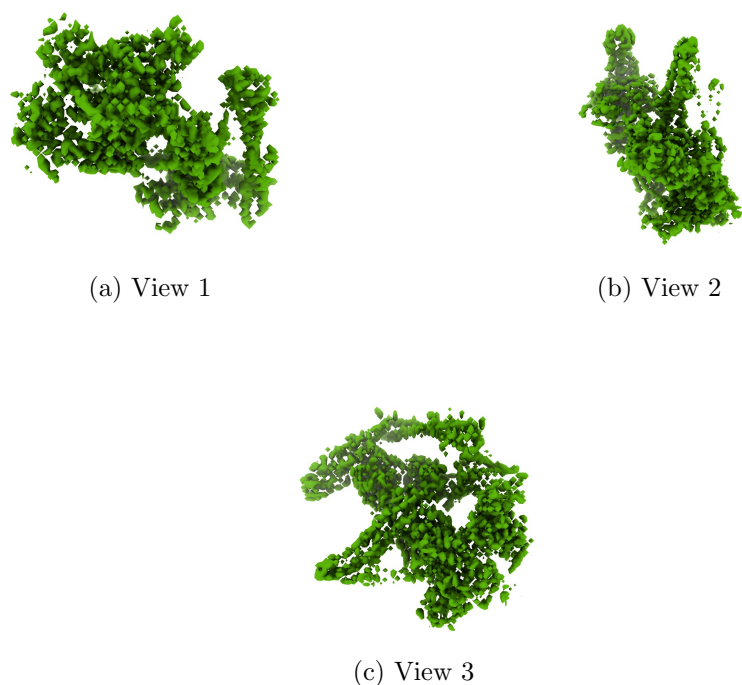
Figure 4: Isosurface at threshold=0.154000. Views generated by ChimeraX at a the following X, Y, Z angles: View 1 (0, -90, -90), View 2 (-90, 0, -90), View 3 (0, 0, 0).
