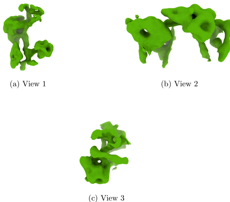
Figure 4: Isosurface at threshold=0.006660. Views generated by ChimeraX at a the following X, Y, Z angles: View 1 (0, -90, -90), View 2 (-90, 0, -90), View 3 (0, 0, 0).
