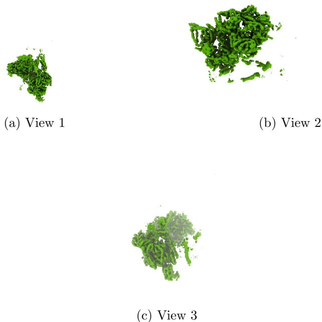
Figure 4: Isosurface at threshold=0.189000. Views generated by ChimeraX at a the following X, Y, Z angles: View 1 (0, -90, -90), View 2 (-90, 0, -90), View 3 (0, 0, 0).
