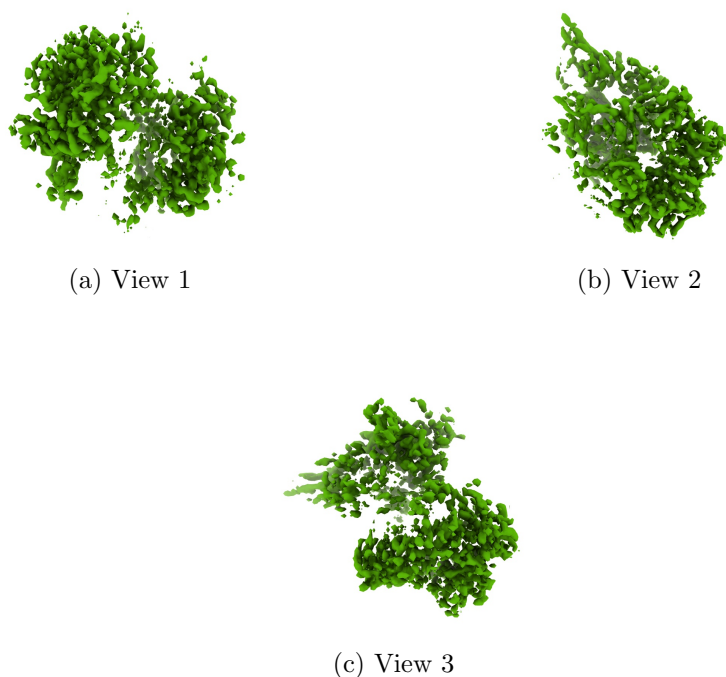
Figure 4: Isosurface at threshold=0.275000. Views generated by ChimeraX at a the following X, Y, Z angles: View 1 (0, -90, -90), View 2 (-90, 0, -90), View 3 (0, 0, 0).
