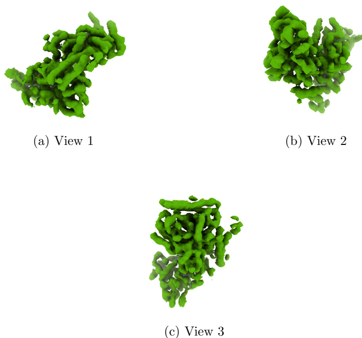
Figure 4: Isosurface at threshold=0.145000. Views generated by ChimeraX at a the following X, Y, Z angles: View 1 (0, -90, -90), View 2 (-90, 0, -90), View 3 (0, 0, 0).
