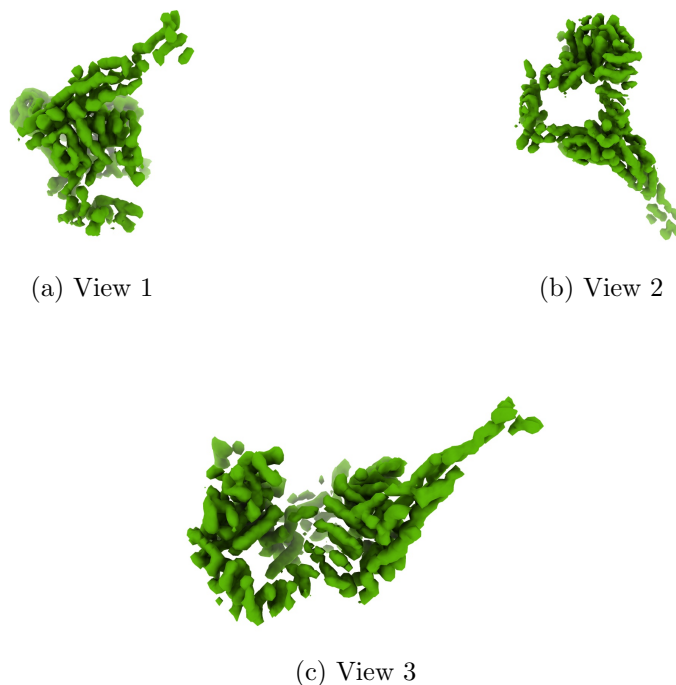
Figure 4: Isosurface at threshold=0.152000. Views generated by ChimeraX at a the following X, Y, Z angles: View 1 (0, -90, -90), View 2 (-90, 0, -90), View 3 (0, 0, 0).
