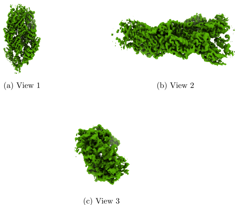
Figure 4: Isosurface at threshold=0.173000. Views generated by ChimeraX at a the following X, Y, Z angles: View 1 (0, -90, -90), View 2 (-90, 0, -90), View 3 (0, 0, 0).
