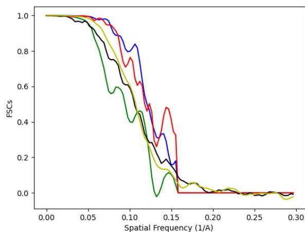
Figure 25: FSC in X, Y, Z, the global FSC, and the Average Cosine Phase.
