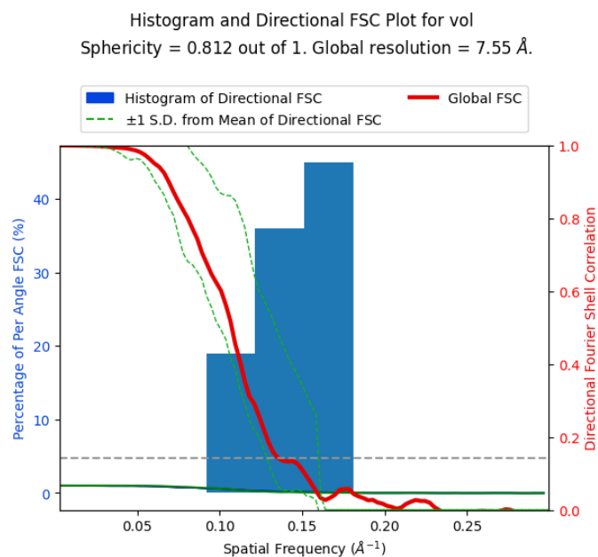
Figure 26: Global FSC and histogram of the directional FSC.
