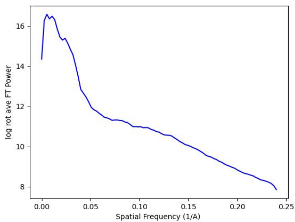
Figure 27: Logarithm of the radial average of the input map power in Fourier space.
