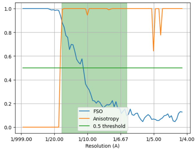
Figure 23: FSO and anisotropy.
