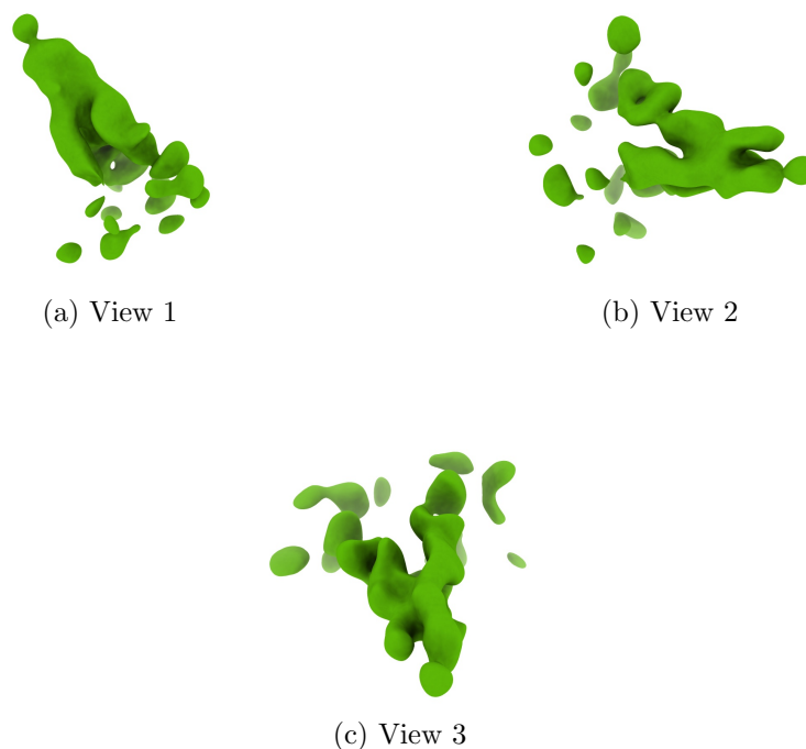
Figure 4: Isosurface at threshold=0.011500. Views generated by ChimeraX at a the following X, Y, Z angles: View 1 (0, -90, -90), View 2 (-90, 0, -90), View 3 (0, 0, 0).
