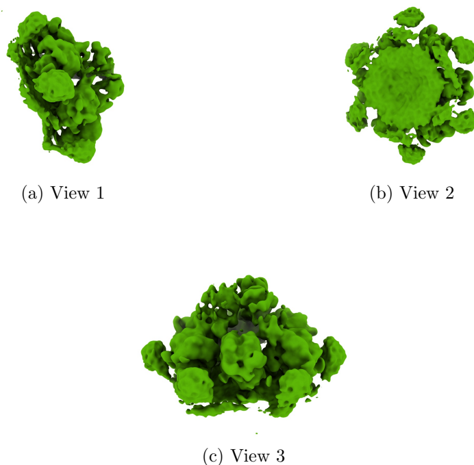
Figure 4: Isosurface at threshold=0.012000. Views generated by ChimeraX at a the following X, Y, Z angles: View 1 (0, -90, -90), View 2 (-90, 0, -90), View 3 (0, 0, 0).
