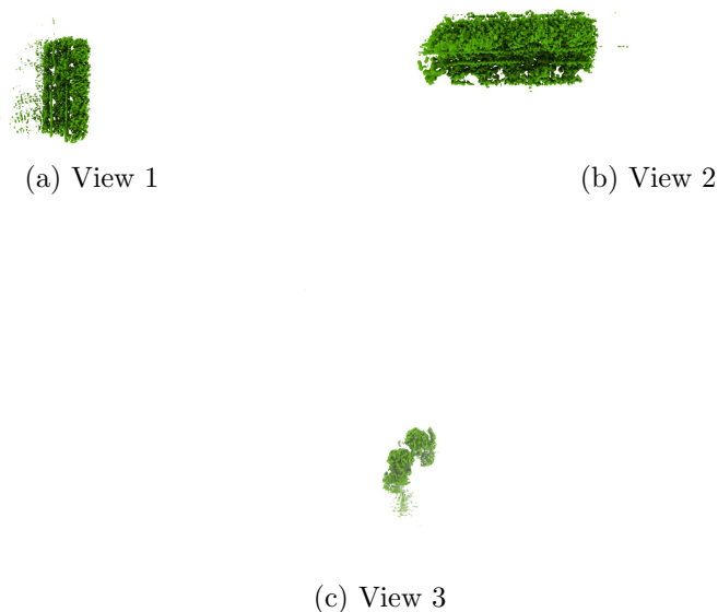
Figure 4: Isosurface at threshold=0.162000. Views generated by ChimeraX at a the following X, Y, Z angles: View 1 (0, -90, -90), View 2 (-90, 0, -90), View 3 (0, 0, 0).
