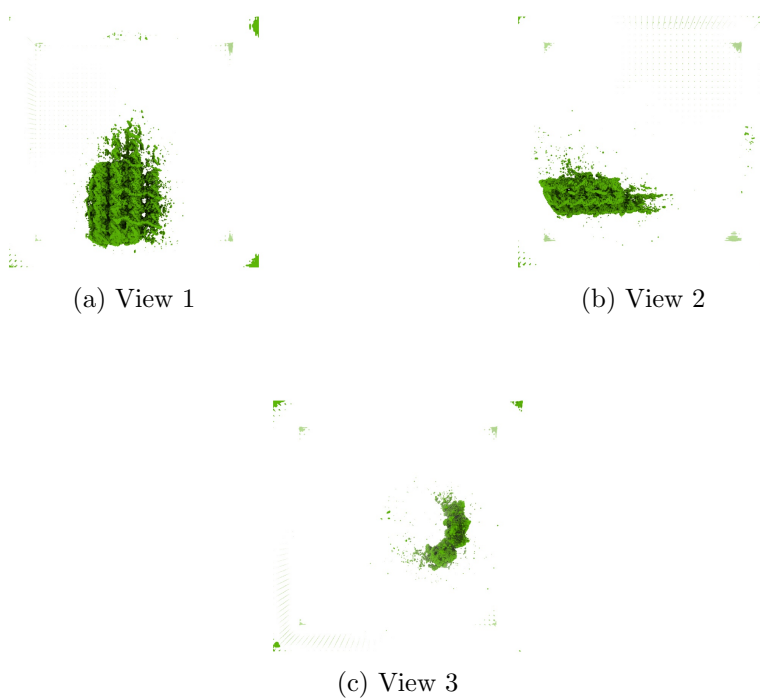
Figure 4: Isosurface at threshold=0.000178. Views generated by ChimeraX at a the following X, Y, Z angles: View 1 (0, -90, -90), View 2 (-90, 0, -90), View 3 (0, 0, 0).
