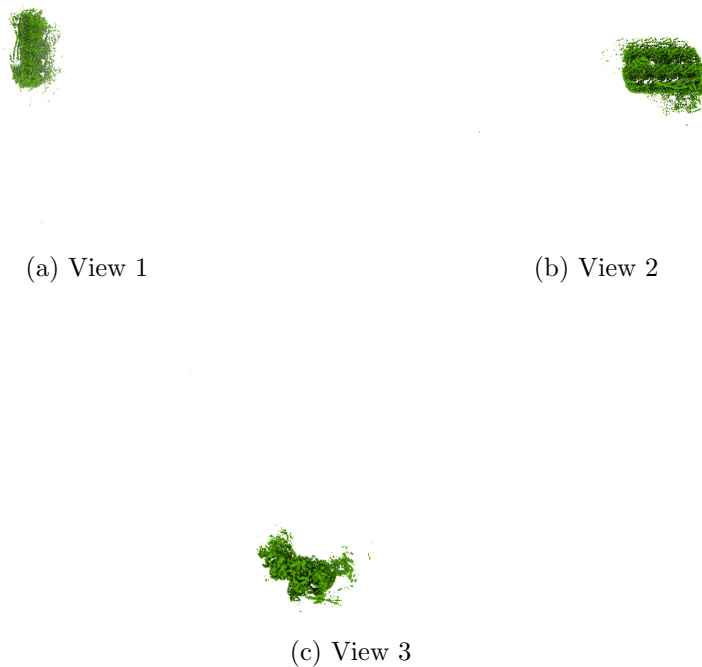
Figure 4: Isosurface at threshold=0.164000. Views generated by ChimeraX at a the following X, Y, Z angles: View 1 (0, -90, -90), View 2 (-90, 0, -90), View 3 (0, 0, 0).
