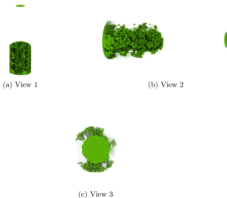
Figure 4: Isosurface at threshold=0.004080. Views generated by ChimeraX at a the following X, Y, Z angles: View 1 (0, -90, -90), View 2 (-90, 0, -90), View 3 (0, 0, 0).
